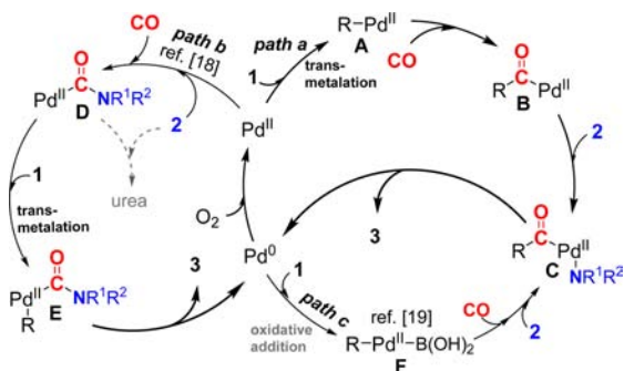
Scheme 6. Proposed Comprehensive Mechanism
